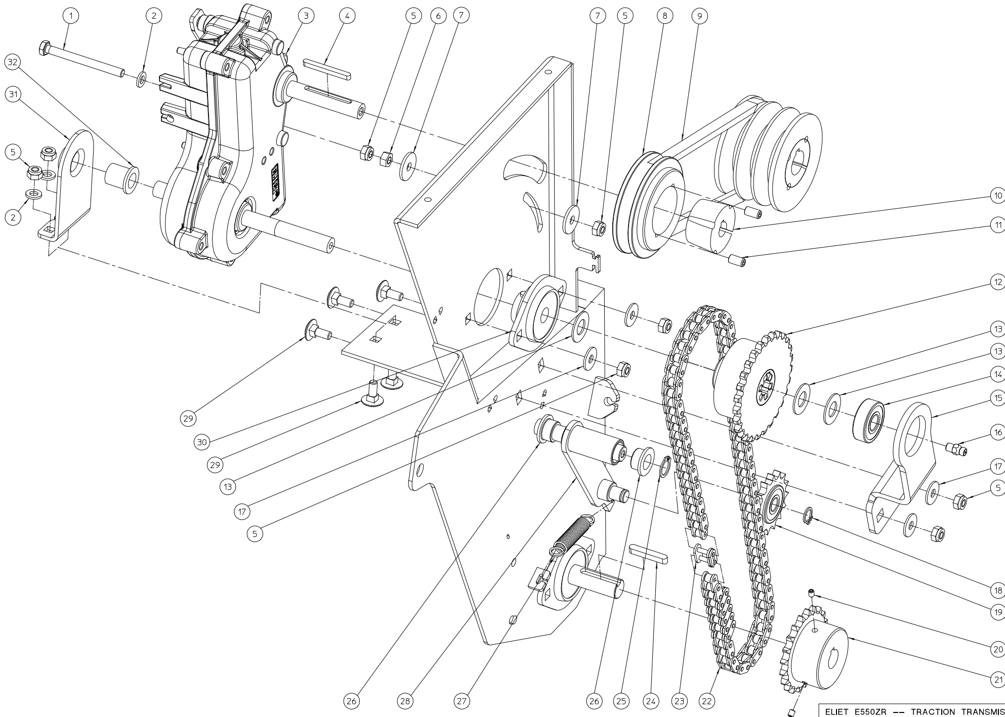
ELIET E550ZR -- TRACTION TRANSMISSION
